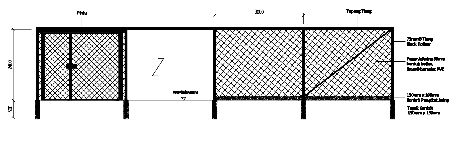
PANDANGAN HADAPAN
